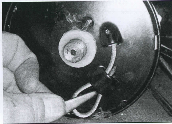
Reinstall retaining pin after the floating safety stop is installed on wire rope. Tap in place with punch or screwdriver.
