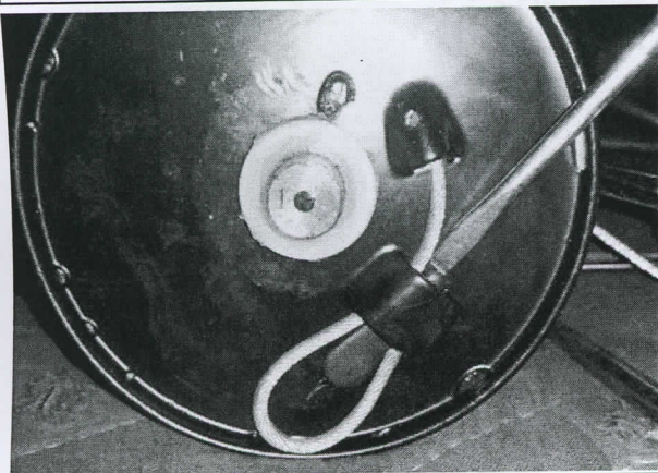
Remove retaining pin with punch or screwdriver.
