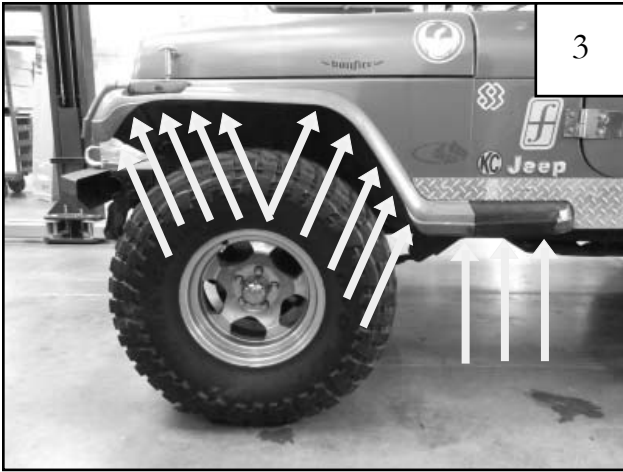
Remove the factory installed fender flare and rocker guard screws with a socket wrench. (12 total locations) 9 on main flare (use 5/16" socket), 3 on rocker panel (use 3/8" socket)
